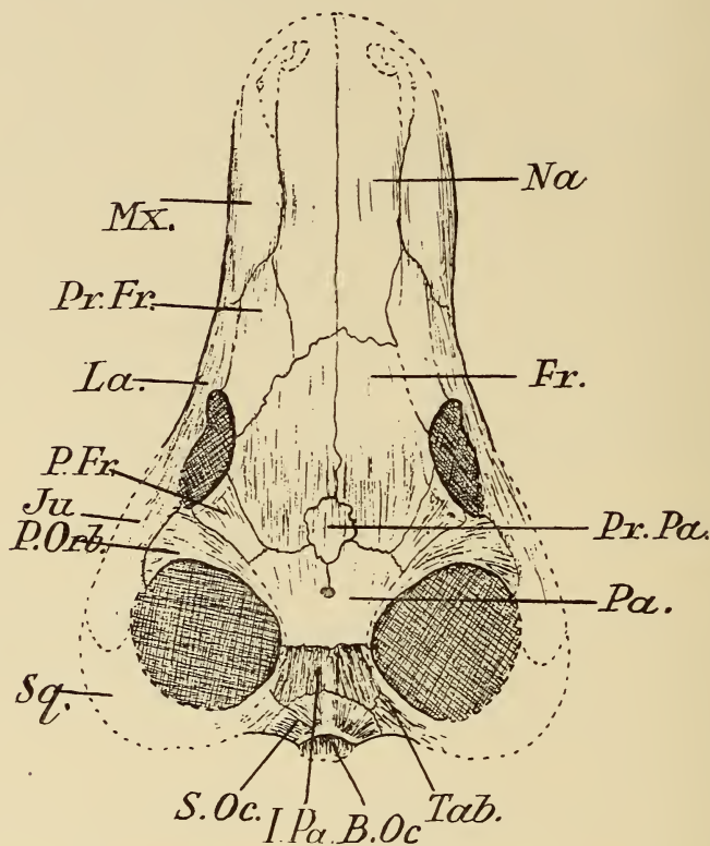
FIG. 11.— Cynariops robustus . Type, B.M.N.H., R5743. Dorsal view of the skull. \times \frac{5}{7} .
